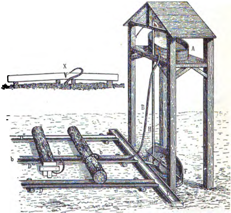
Fig. 308.—French method of injection. After Boppe.
